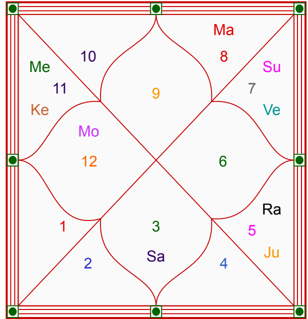
Navamsa Chart
